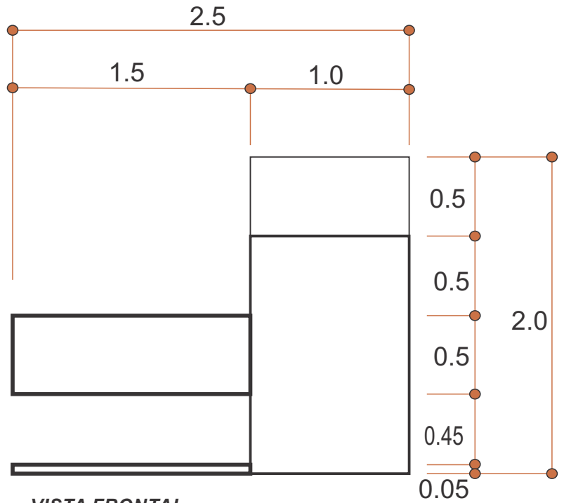
VISTA FRONTAL
